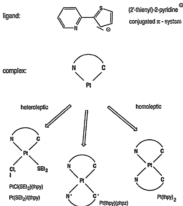
Fig. 1. The 2-(2'-thienyl)pyridine anion and some of its Pt(II)-complexes.
