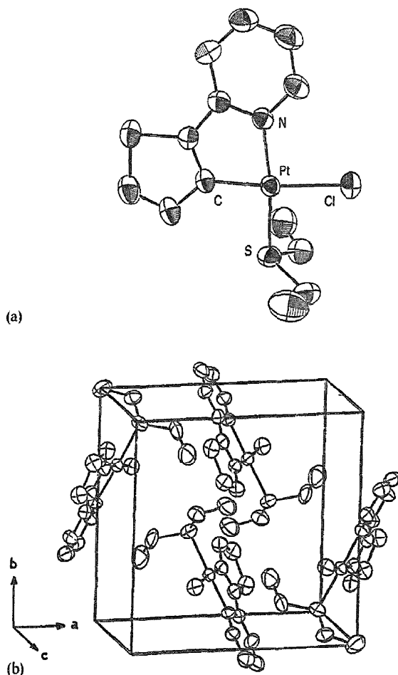
Fig. 2. Molecular structure (a) and unit cell (b) of PtCl(Et 2 S)(thpy) (Ortep plots).
